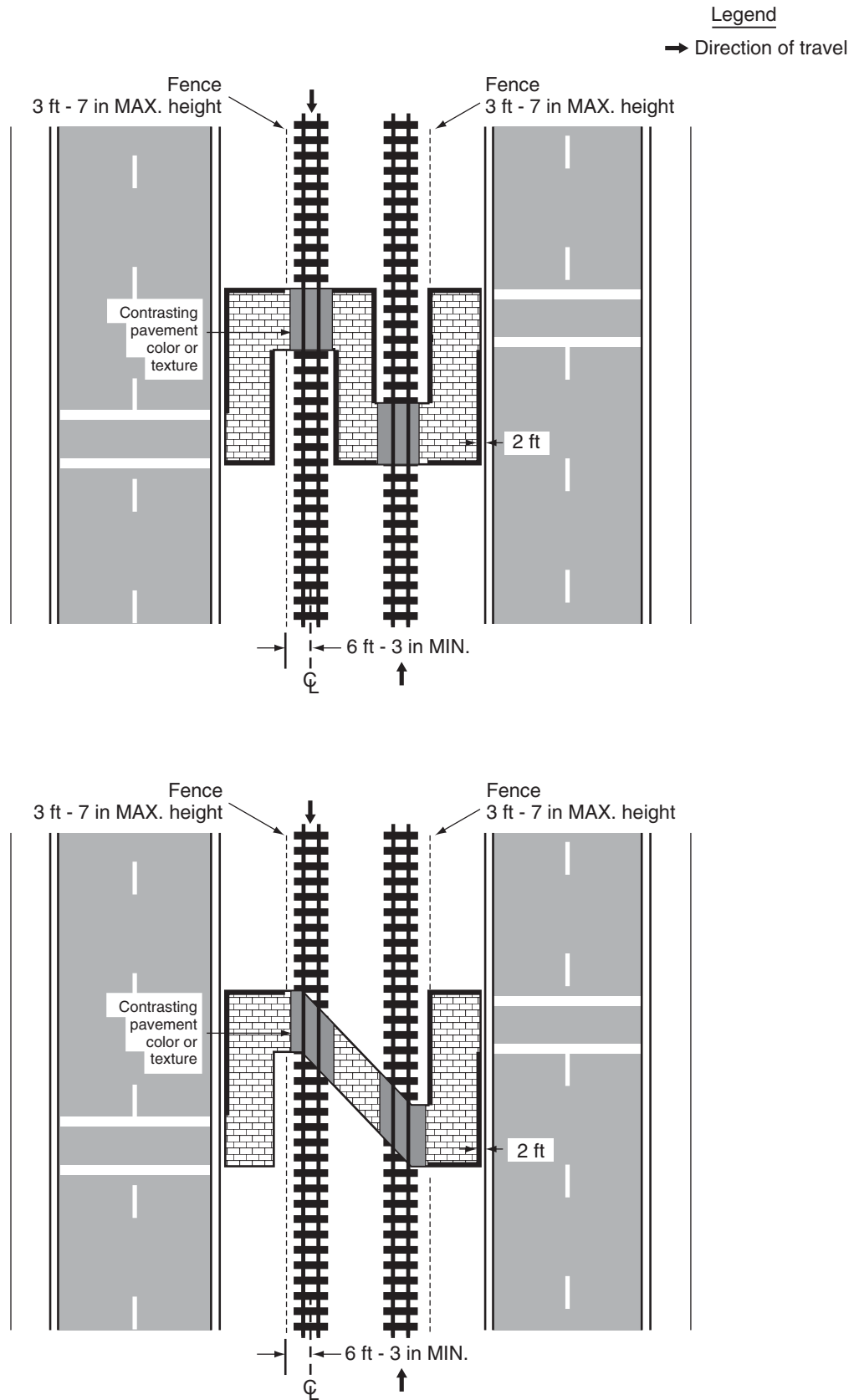
Figure 10D-8. Examples of Pedestrian Barrier Installation at an Offset Nonintersection Light Rail Transit Crossing
