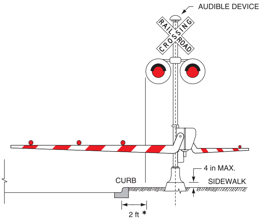
Figure 10D-4. Example of Pedestrian Gate Placement with Pedestrian Gate Arm
