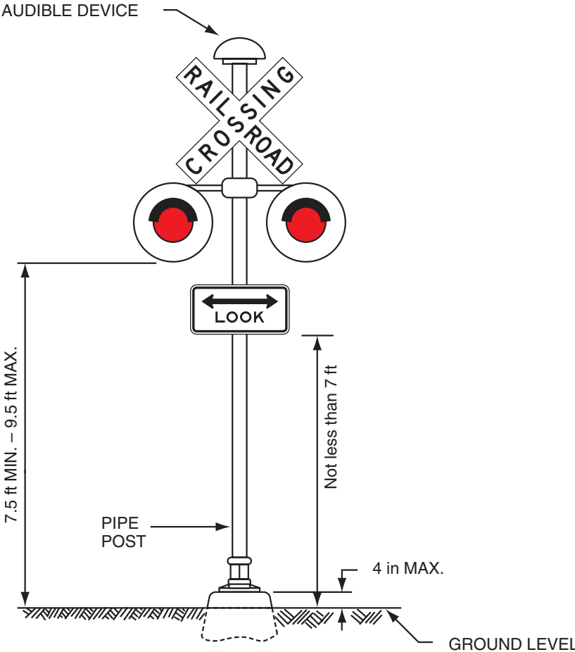
Figure 10D-2. Example of Light Rail Transit Flashing-Light Signal Assembly for Pedestrian Crossings
